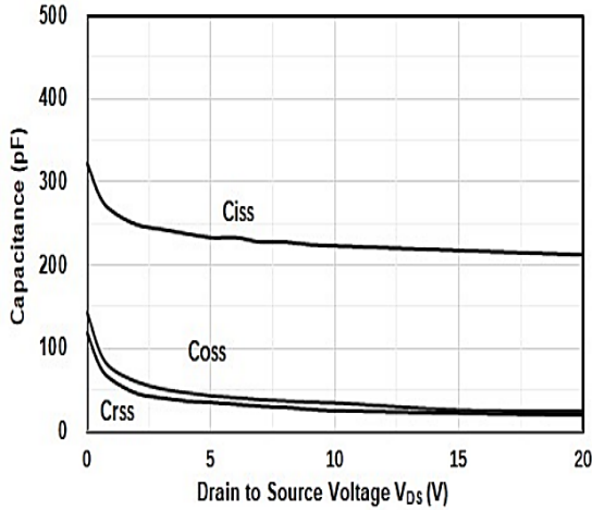
Figure3. Capacitance Characteristics
